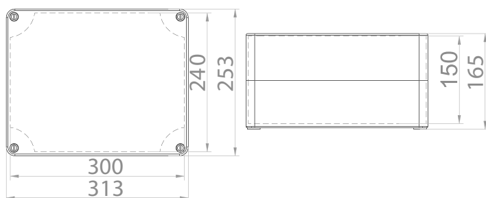
Krabice SolidBOX IP65 / Sealed box IP65 - Obj.č. / Item 68250 / 68251
