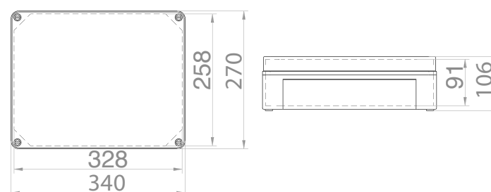
Krabice SolidBOX IP65 / Sealed box IP65 - Obj.č. / Item 68250 / 68251
