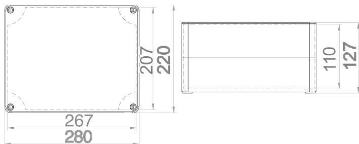
Krabice SolidBOX IP65 / Sealed box IP65 - Obj.č. / Item 68220
