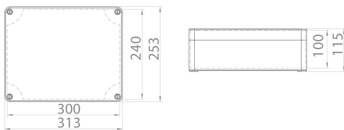
Krabice SolidBOX IP65 / Sealed box IP65 - Obj.č. / Item 68230 / 68231
